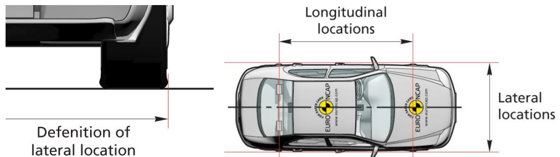
Figure 6-3: Vehicle dimensional measurements
